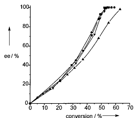
Figure 1. Plot of ee [%] against conversion [%] for the kinetic resolution of 1a with ( S,R,R )-L1, [Cu(OTf) 2 ] and Et 2 Zn (■), i Pr 2 Zn (▲), n Bu 2 Zn (●), and Me 2 Zn (▼) (entries 1, 13, 14, and 17 in Table 1).
